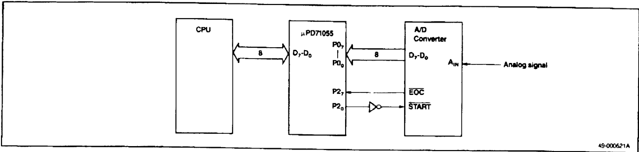
Figure 8. A/D Converter Example
