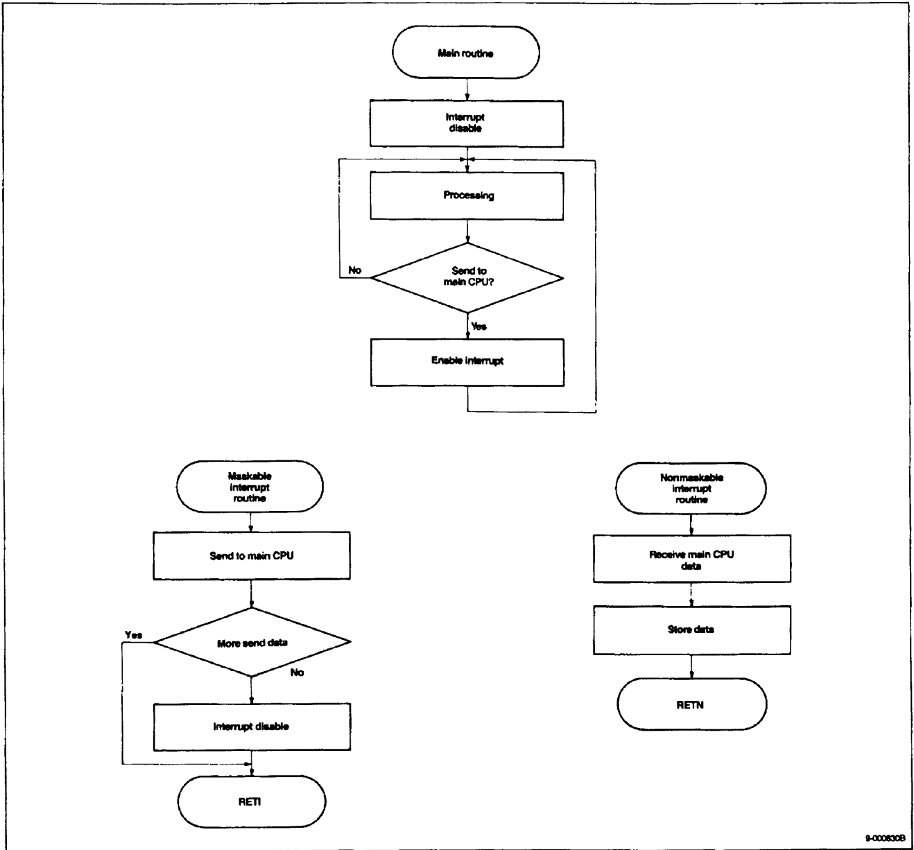
Figure 19. Sub CPU Flowchart
