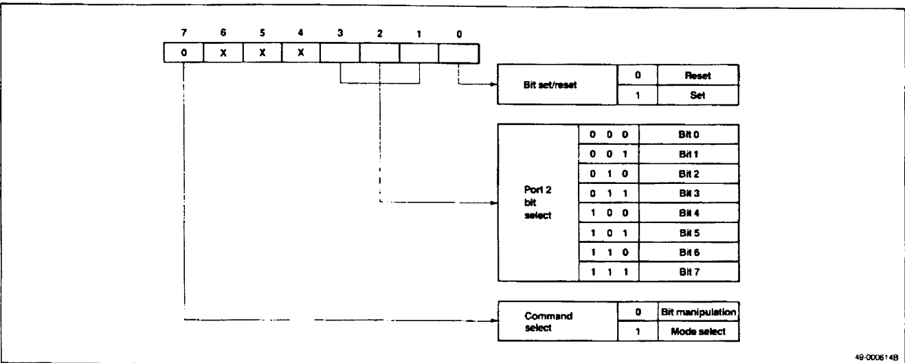
Figure 2. Bit Manipulation Command Word
