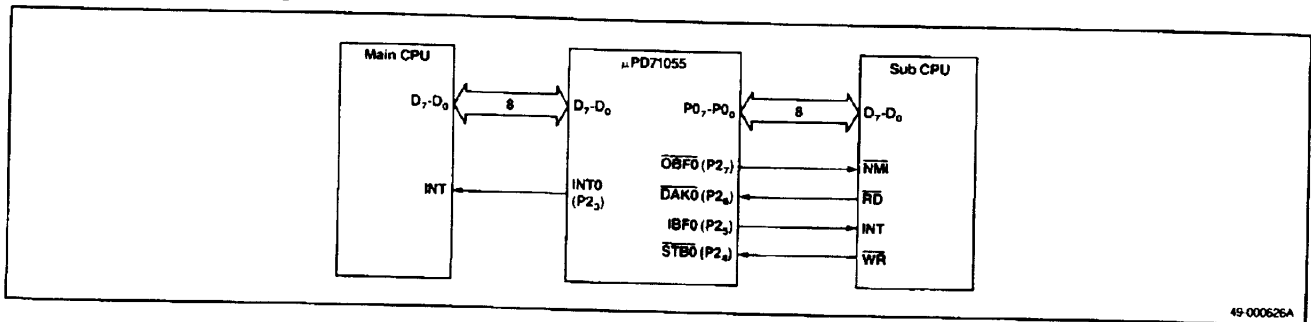
Figure 17. Connecting Two CPUs
