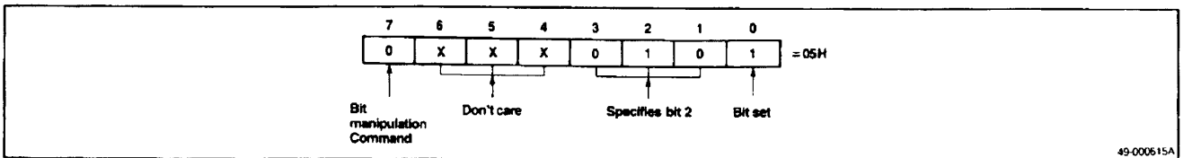
Figure 3. Bit Manipulation Command Example
